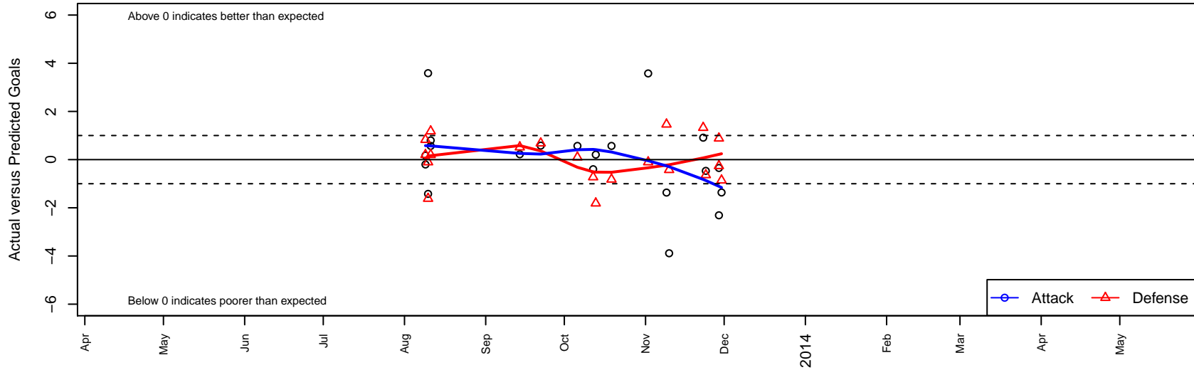
Diablo FC B98 Dots are actual minus expected GF (blue circles) and GA (red triangles). Blue line is smoothed change in attack strength. Red is smoothed change in defense strength.
